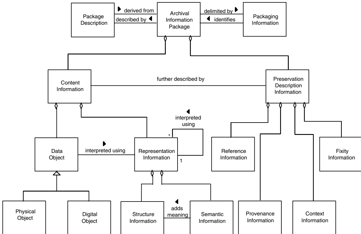
Figure 4-18: Archival Information Package (Detailed View)
