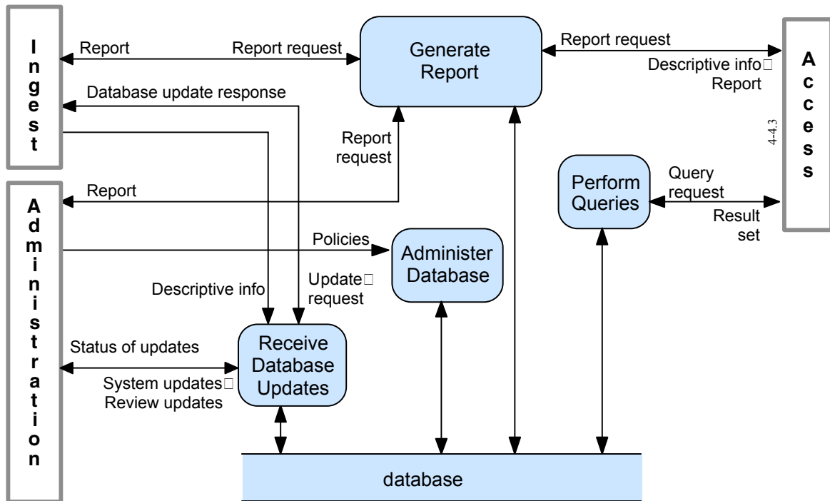
Figure 4-4: Functions of Data Management
