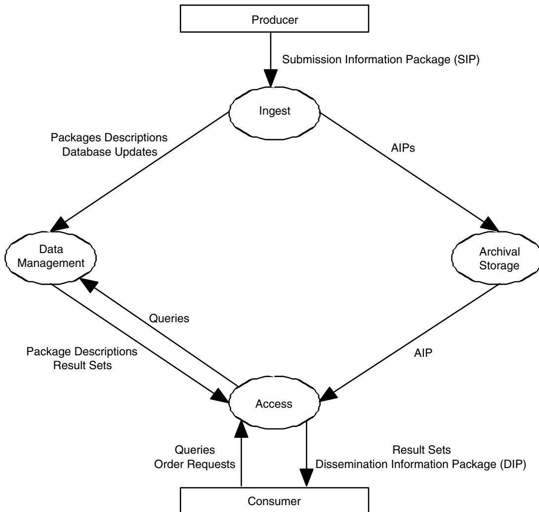
Figure 4-26: High-Level Data Flows in an OAIS
