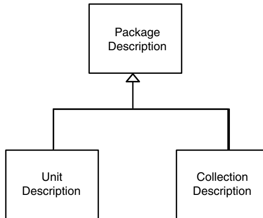
Figure 4-20: Archival Specialization of the Package
