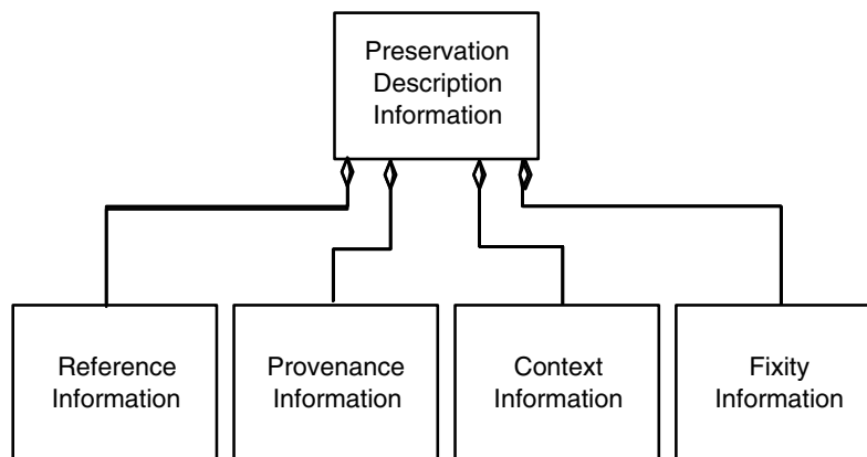
Figure 4-16: Preservation Description Information (PDI)
