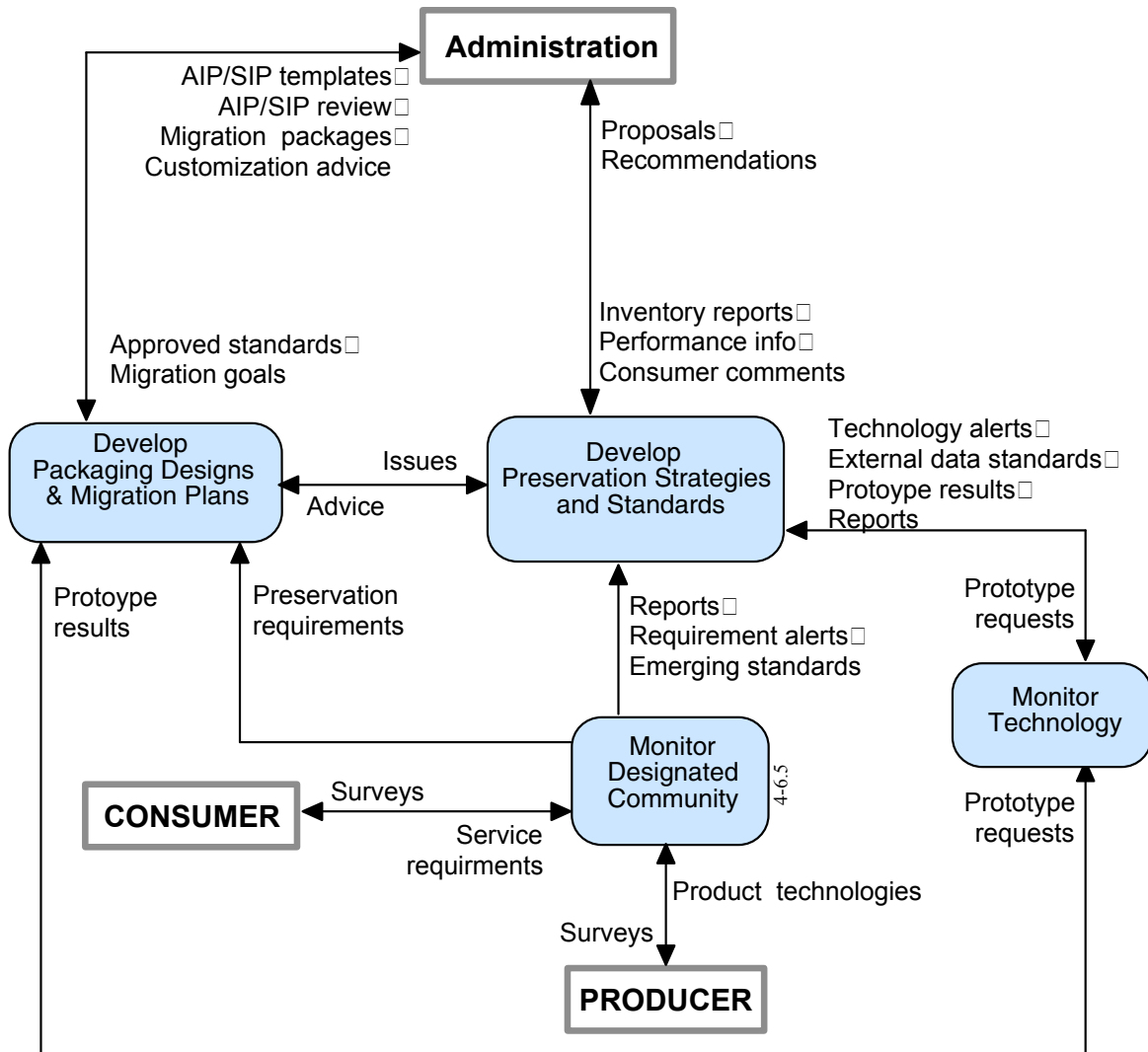
Figure 4-6: Functions of Preservation Planning
