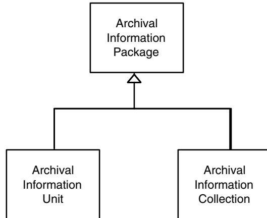
Figure 4-19: Archival Specialization of the AIP
