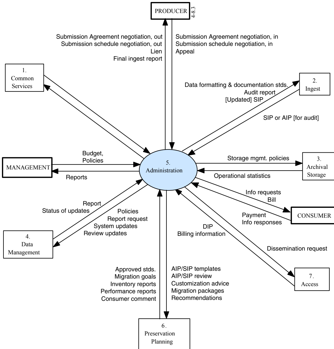
Figure 4-9: Administration Context Diagram
