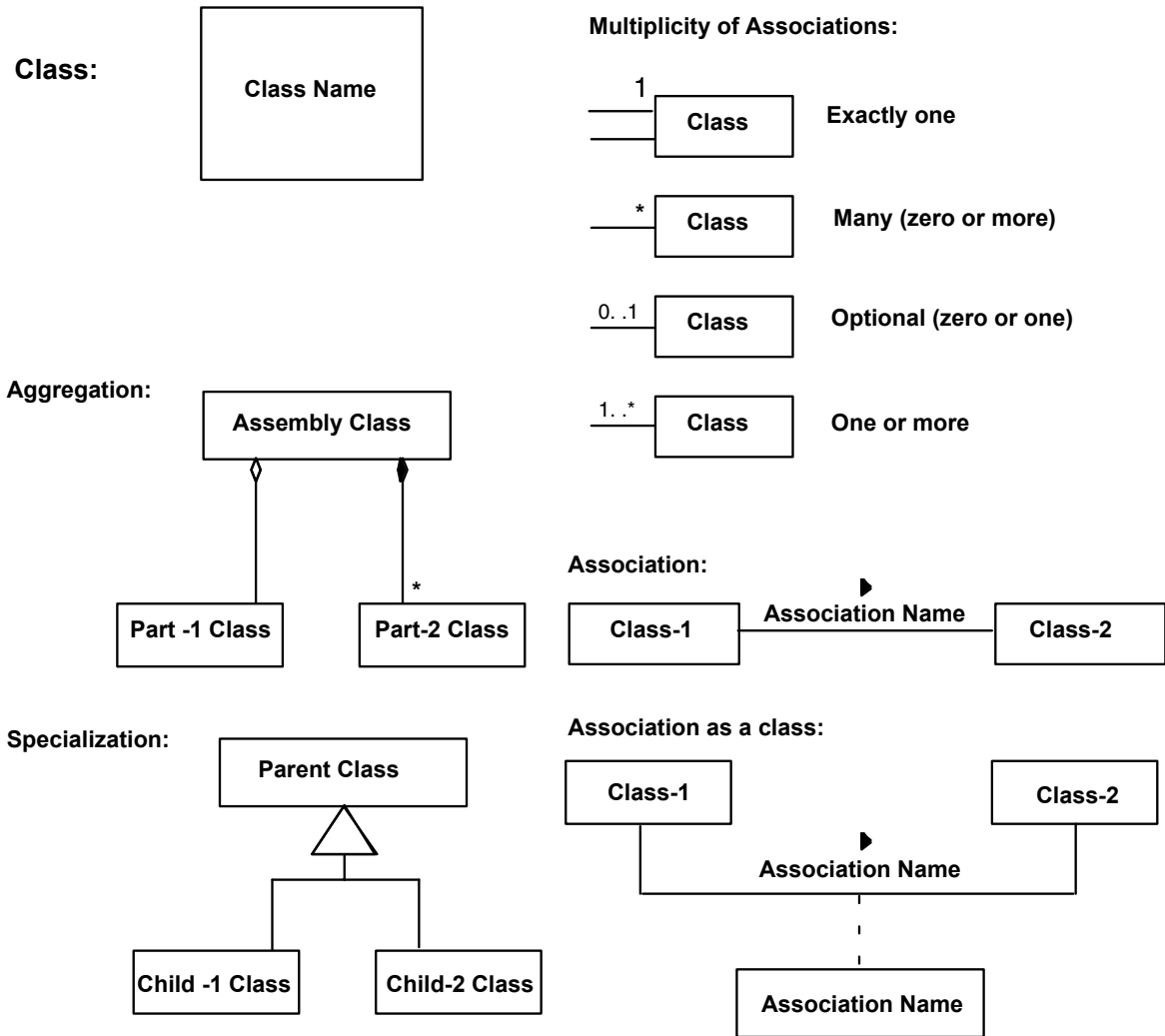
Figure C-1: Key to UML Relationships
