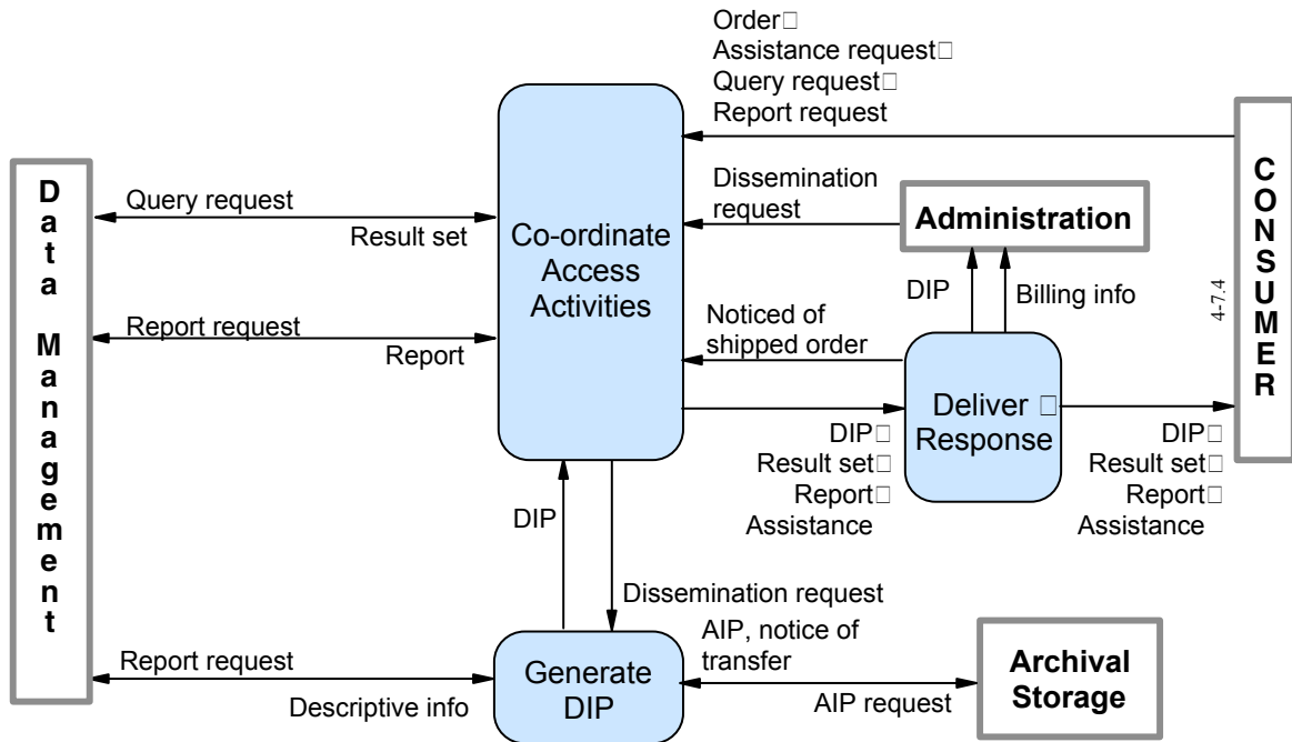
Figure 4-7: Functions of Access
