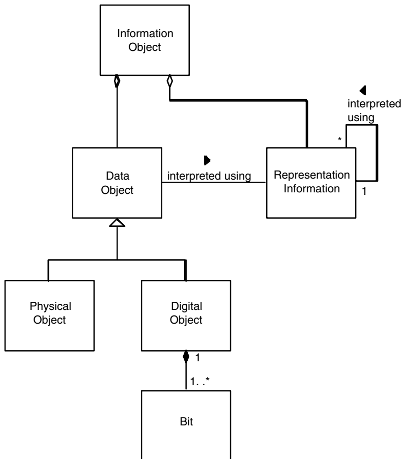
Figure 4-10: Information Object
