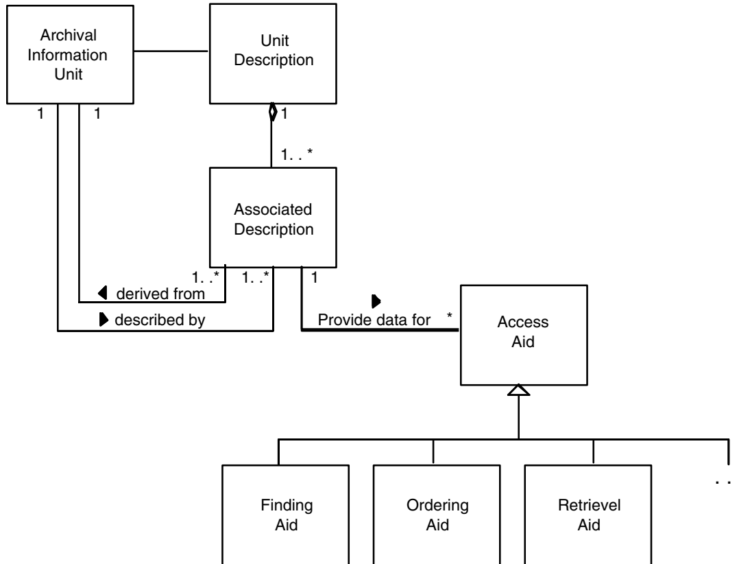
Figure 4-22: Unit Description
