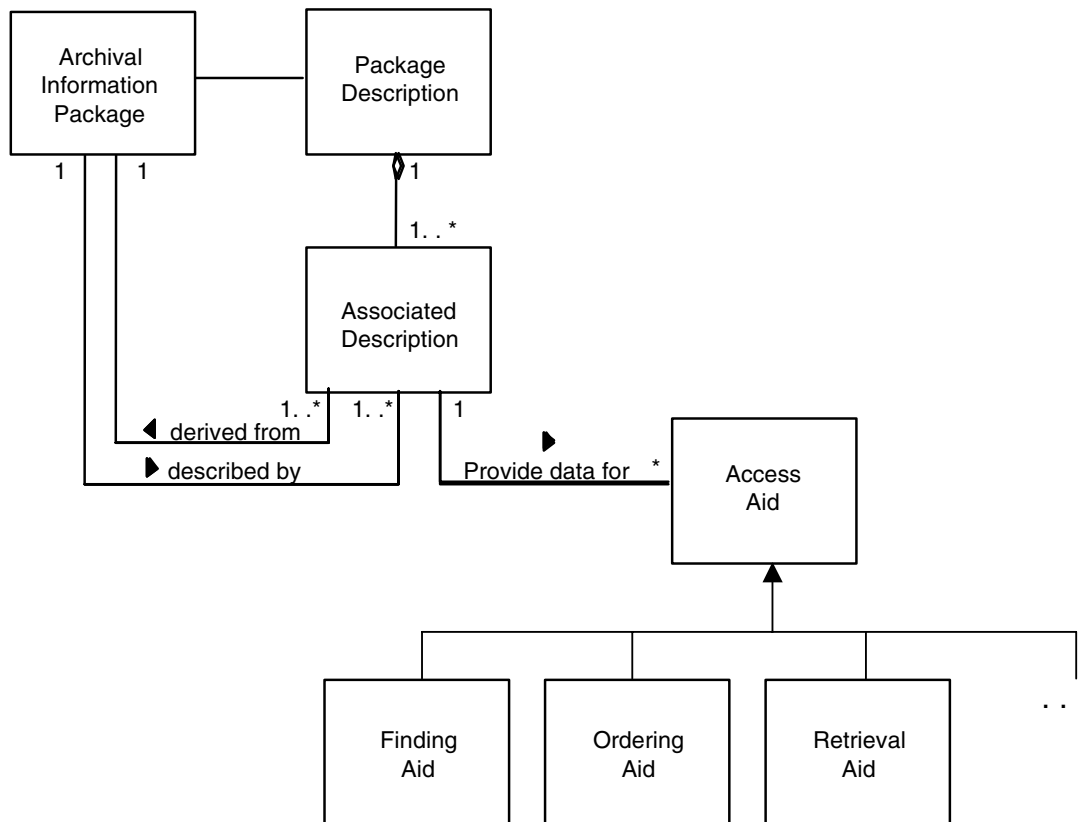
Figure 4-17: Package Description
